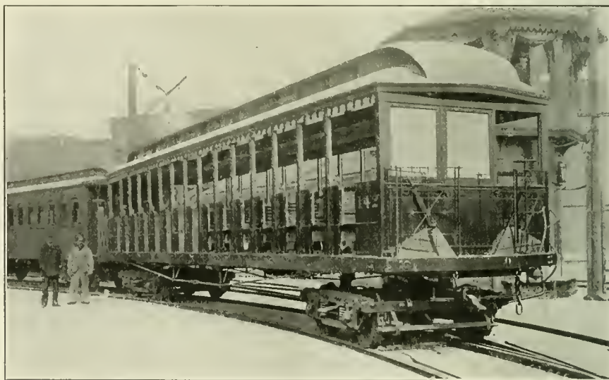
STANDARD OPEN CAR, MANHATTAN ELEVATED RAILWAY.
